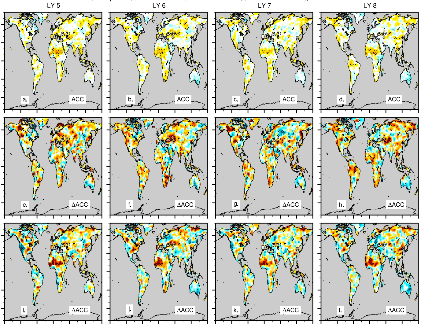
ACC, Precipitation, OBS=CRU-TS4.0, Season=ANNUAL, (LY 5: 1959.5-2015.5), detrended
