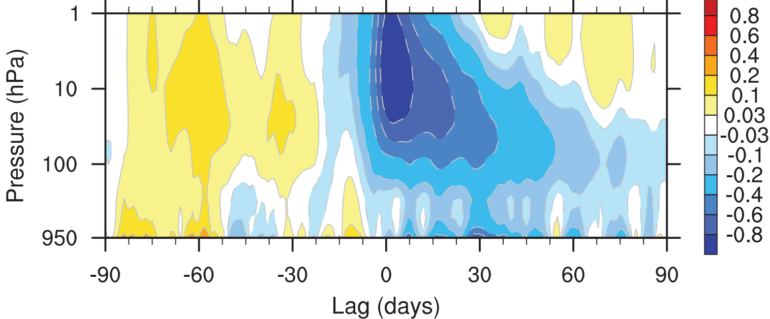
CAM5-L46 NAM-Pres index composite (23 SSWs)
