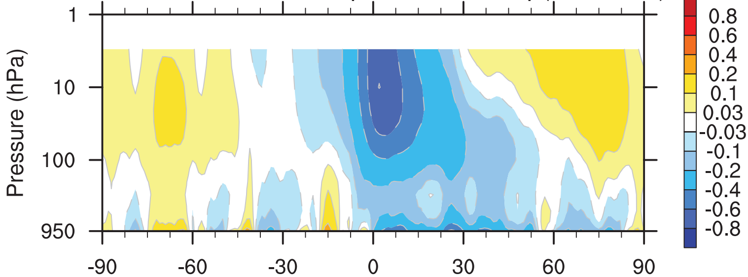
CAM5-L30-GWD NAM-pres index comp(34 SSWs)
