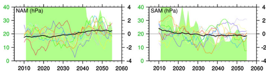
Fig. 5 Ten-year running mean DJF time series of the NAM ( left ) and SAM ( right ), defined as the zonally-averaged SLP anomaly difference between high ( 55^{\circ} – 90^{\circ} ) and middle latitudes ( 30^{\circ} – 55^{\circ} ) of the northern and southern hemisphere, respectively. The thick black
