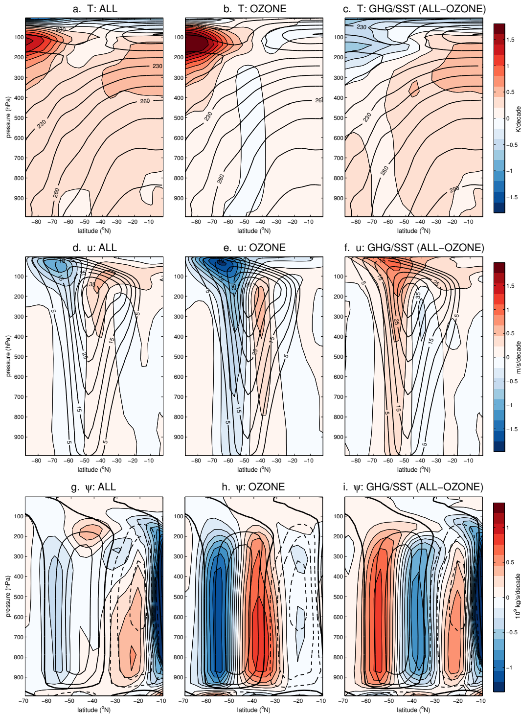
Figure 1. Ensemble mean, zonal mean DJF temperature (top), zonal wind (middle) and mass streamfunction (bottom) responses, during 2001-2060, for the integrations in the ALL ensemble (left), the OZONE ensemble (middle) and their difference (right). Contour intervals are, top to bottom: 0.2^{\circ} K/decade, 0.22 m/s/decade, and 0.25 \times 10^9 kg/s/decade. Black contours: the climatological mean (2001-2010), with contour intervals of 10^{\circ} K, 5 m/s and 1.5 \times 10^{10} kg/s, respectively, and negative contours dashed (and thicker zero contour).
