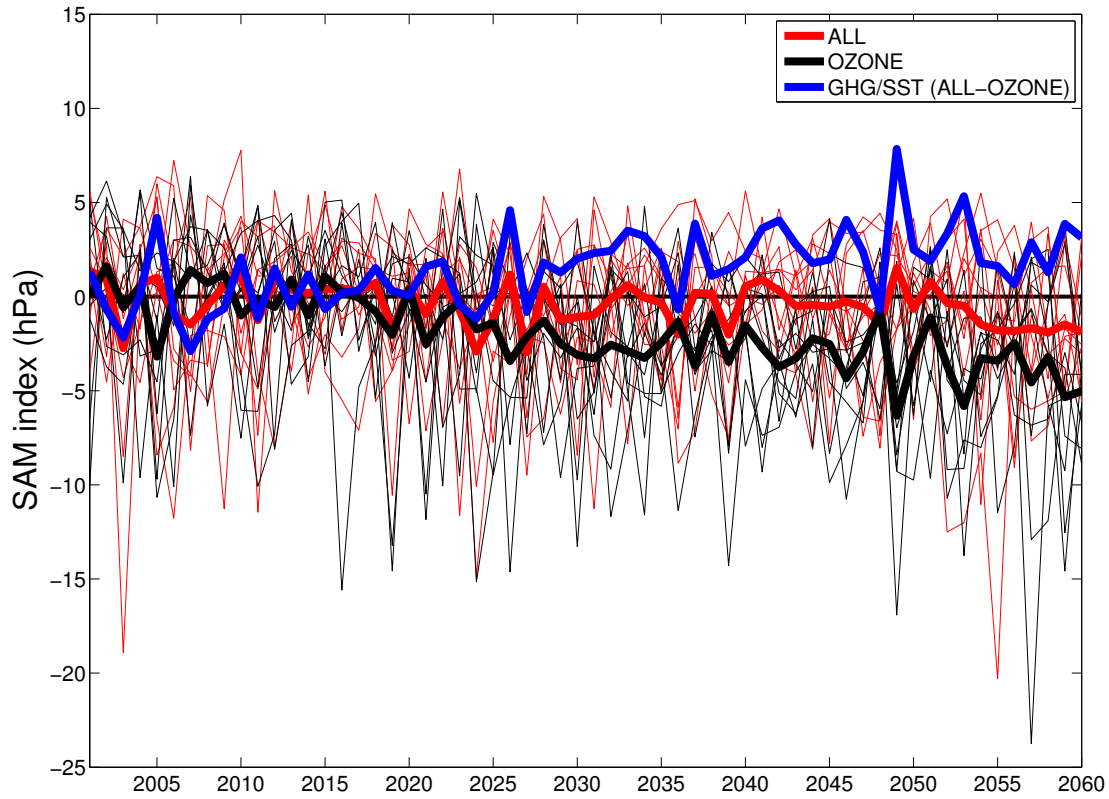
Figure 3. SAM index (anomalies from 2001-2010) in DJF for the two, 10-member ensembles. Thin red and black lines: individual members in the ALL and OZONE ensembles, respectively. Thick red and black lines: the corresponding ensemble means. Thick blue line: the difference of the thick red and black lines, i.e. the SAM response due to all forcings other than ozone recovery.
