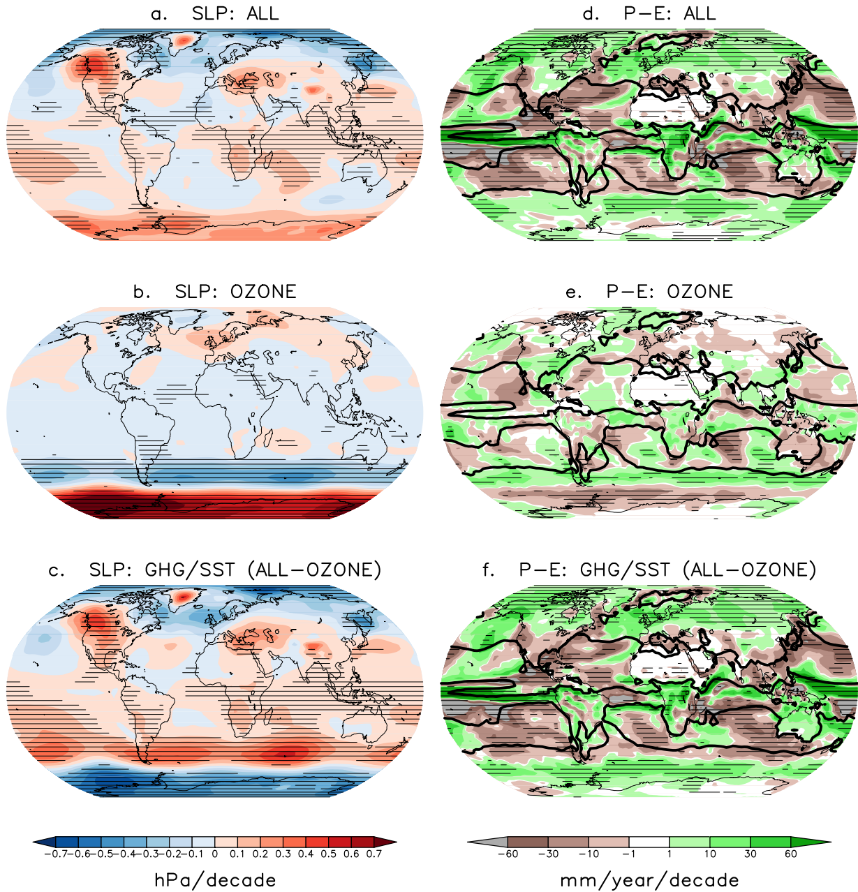
Figure 2. Left column: DJF ensemble mean SLP response, 2001-2060, for the ALL ensemble (top), the OZONE ensemble (middle), and their difference (bottom). Right column: as the left column, but for P - E (thick black lines: climatological mean P - E = 0 during 2001-2010). Statistically significant responses, at the 95% level, are hatched.
