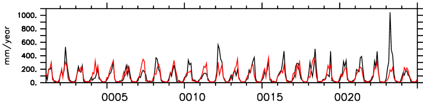
Rainfall at 120W/1N for control (red) and TIW
