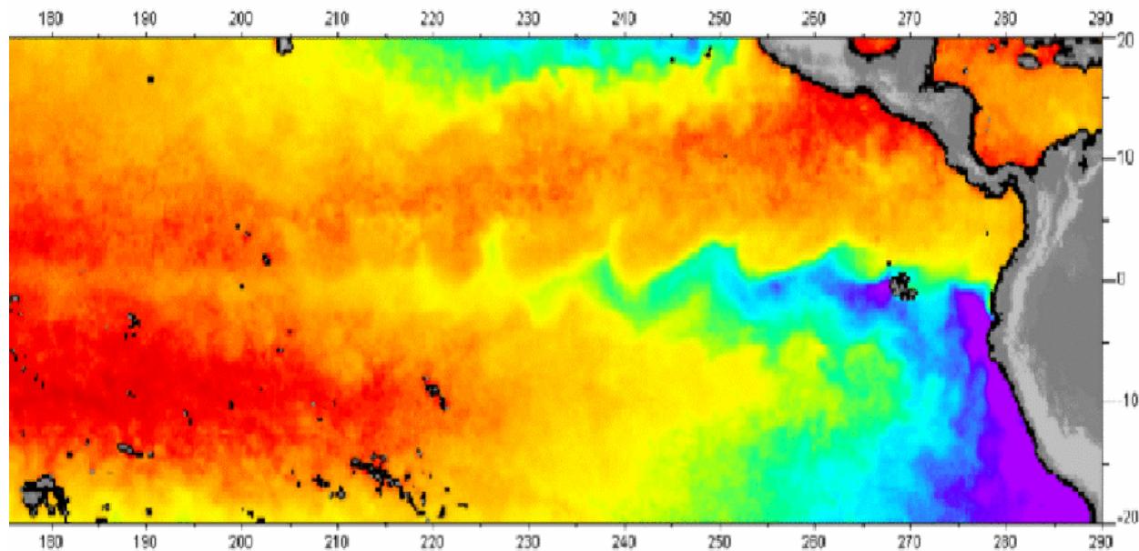
Snapshot of SST on June 2003, from Microwave Imager.
