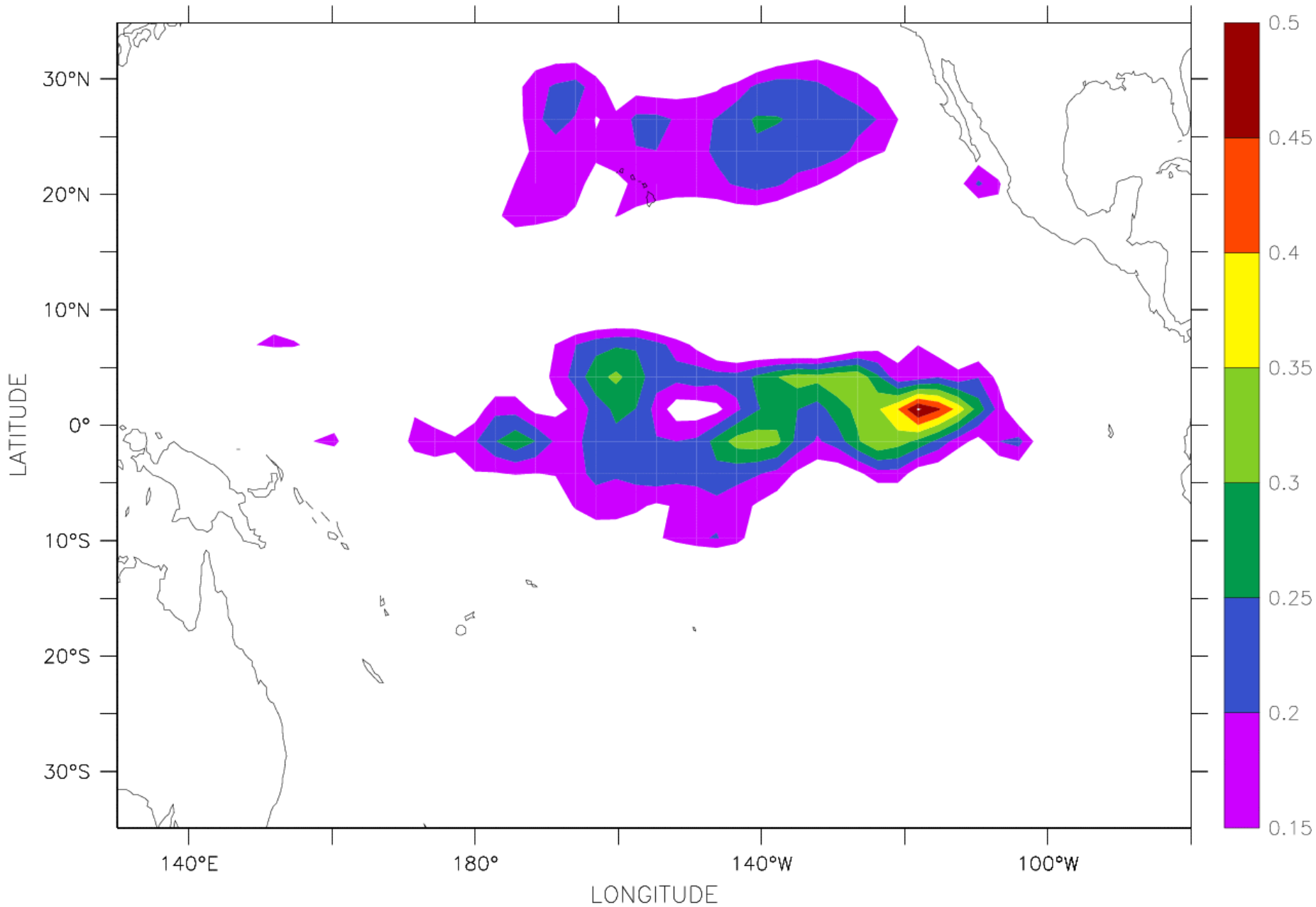
Increase in intraseasonal and interannual wind variability (in %)
